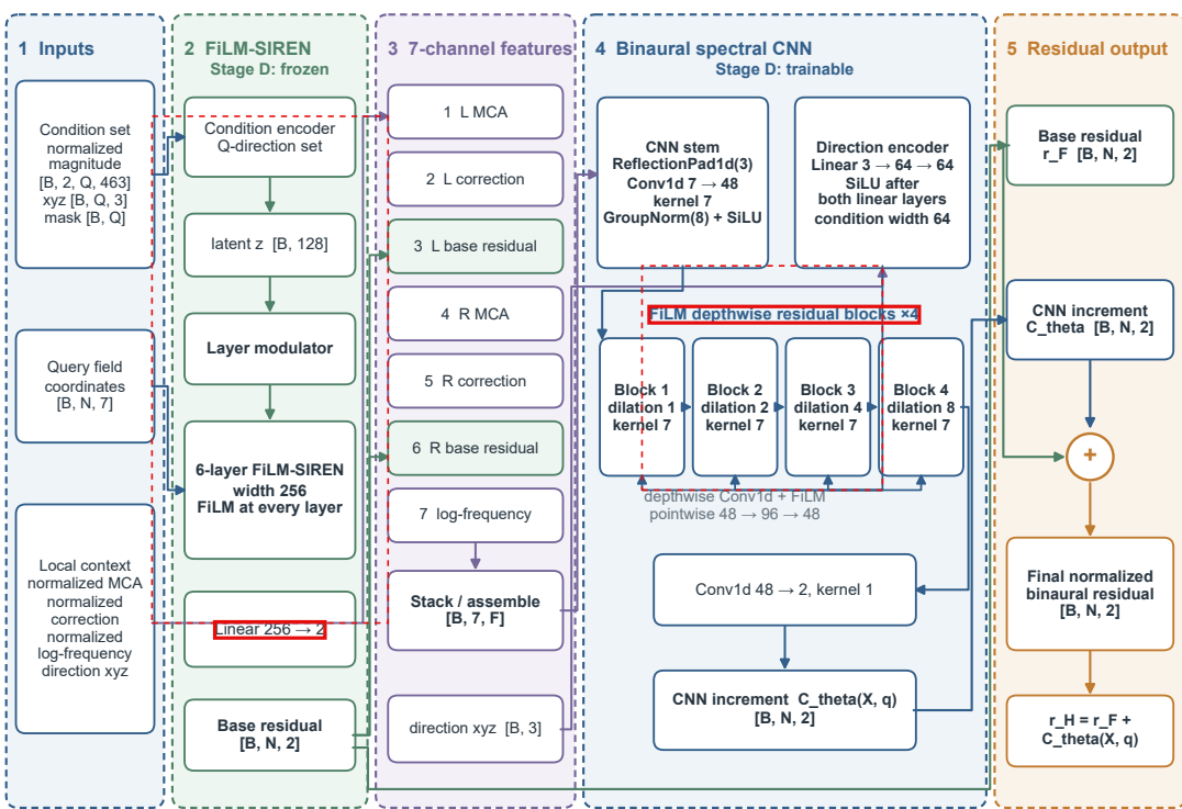
Single prespecified E190 model; the diagram ends at the predicted residual.
